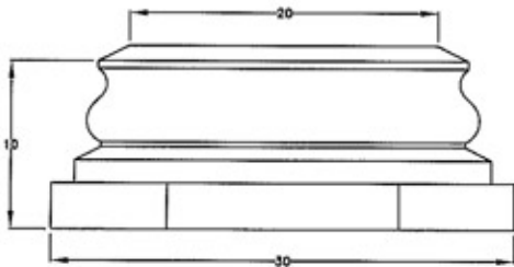
MN0027B
